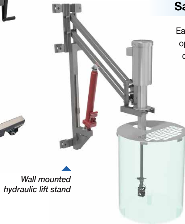
◀ Pilot Mixer lift stand
